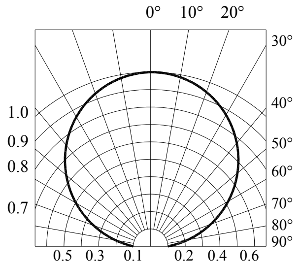
Fig.6 - Radiation Diagram
